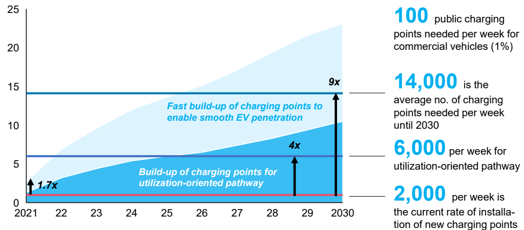
Current vs required weekly public charging point rollout, 2021-30 Number of public AC and DC charging points per week, thousands
